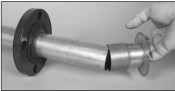
1. Slide flange over pipe and attach CTS Flange Adapter
